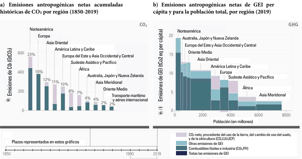
Figure 2.2 (a) and (b) from IPCC, 2023: Current Status and Trends. In: Climate Change 2023: Synthesis Report. Contribution of Working Groups I, II and III to the Sixth Assessment Report of the Intergovernmental Panel on Climate Change [Core Writing Team, H. Lee and J. Romero (eds.)]. IPCC, Geneva, Switzerland, pp. 35-115, doi: 10.59327/IPCC/AR6-9789291691647.
